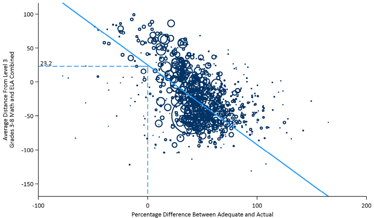
Exhibit 4-17. Scatterplot of Grade 3–8 Test Scores in Relation to the Percentage Difference Between Adequate Cost and Actual Spending
